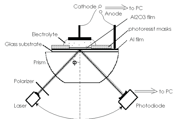
Fig. 8. Scheme of unit for providing of electrochemical oxidation directly on SPR-sensor.
