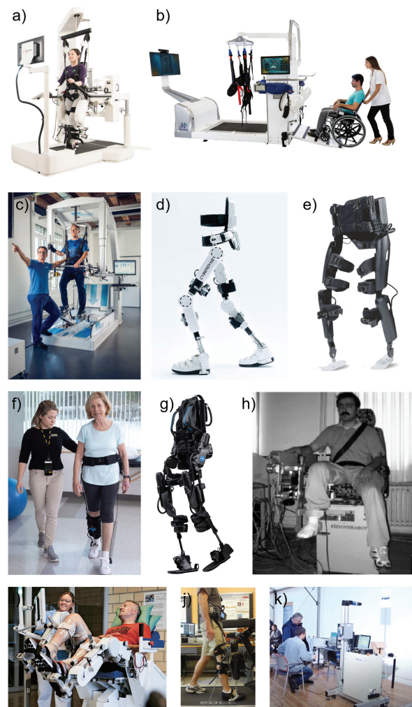
Figure 2. Contemporary rehabilitation robotic systems for lower extremities – a) Lokomat [10], b) ReoAmbulator [15], c) G-EO [16], d) HAL [7], e) ReWalk Personal 6.0 [18], f) ReStore [18], g) EksoNR [5], h) MotionMaker [9], i) Anklebot [20], j) PHYSIOTHERABOT [42], k) RENU-1 [14]
