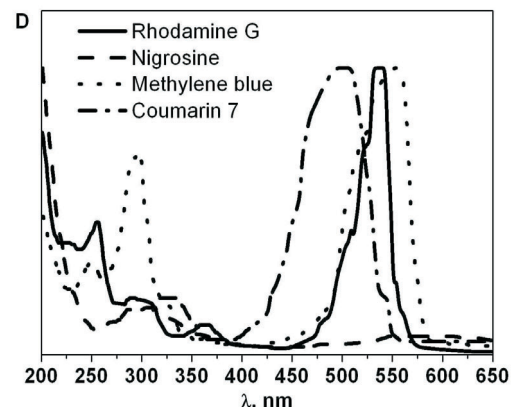
Fig. 1. Absorption spectra of silica sol-gel films doped with organic dyes.
