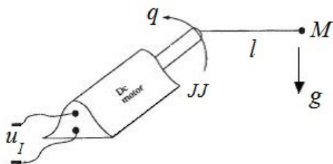
Fig. 1. Schematic of one DOF robot manipulator
