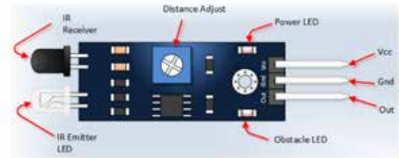
Fig. 8. IR receiver
