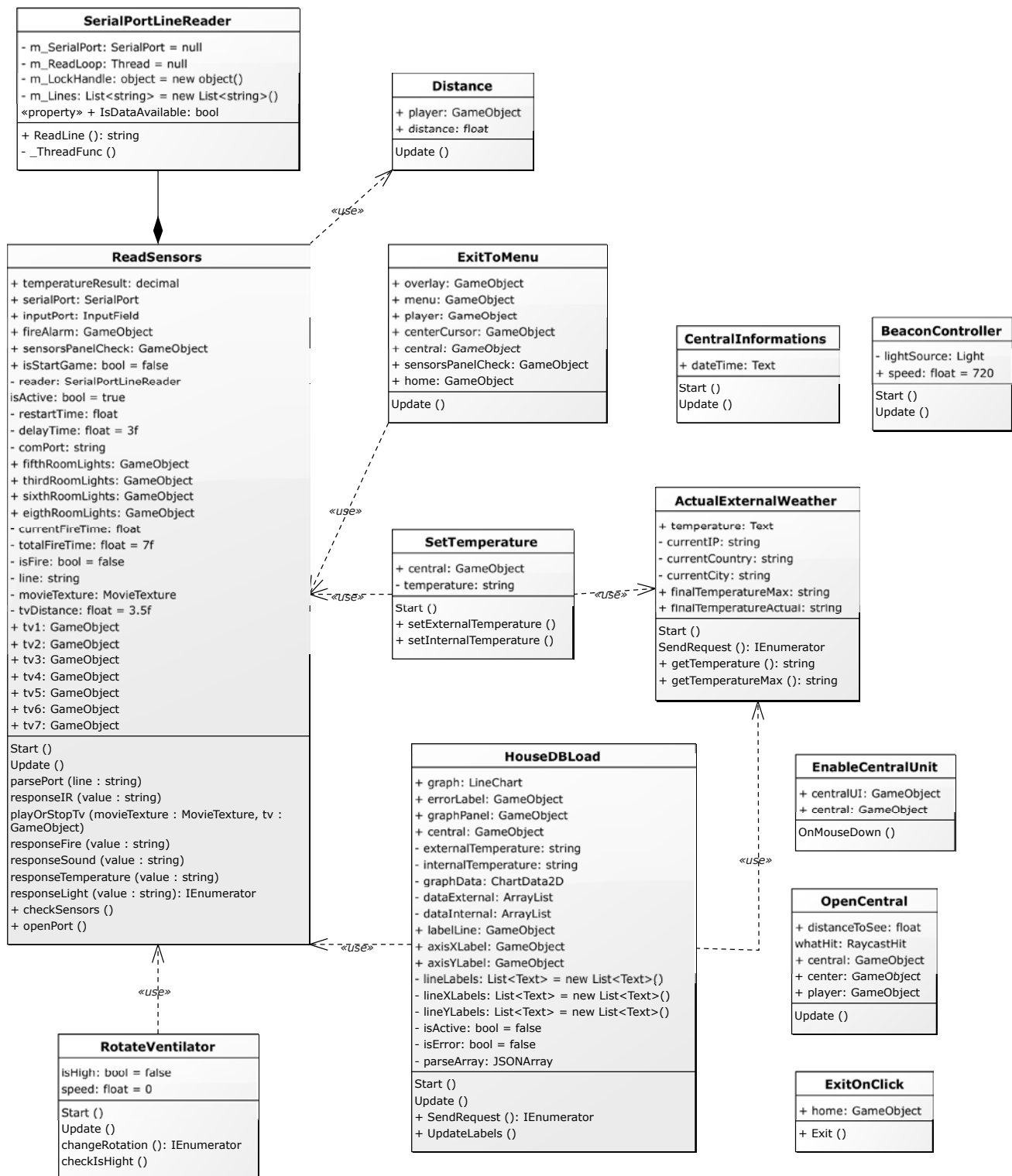
Fig. 11. Class diagram
