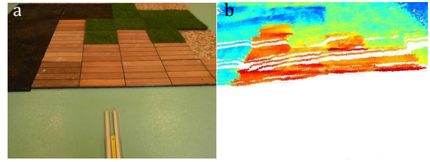
Fig. 7. Intensity values obtained from Hokuyo laser range finder – observed scene (a) and registered intensity values (b)
