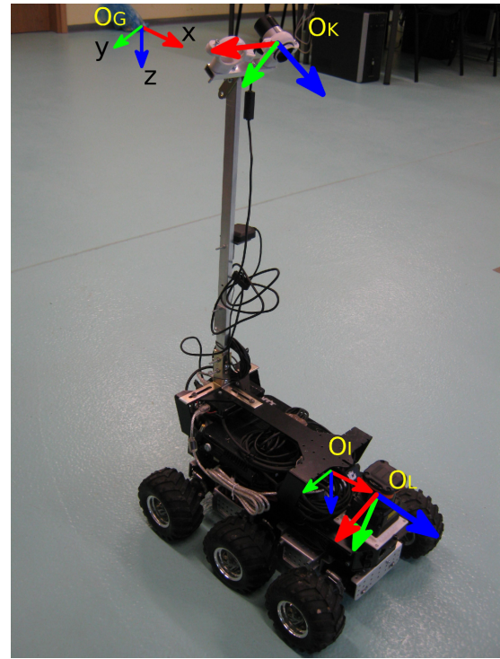
Fig. 1. Configuration of the sensors attached to the robot's platform
