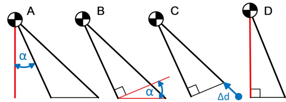
Fig. 7. Illustration of the side fall prevention strategy (from left to right)
