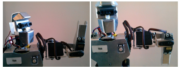
Fig. 5. Approximating human arm configurations with the limited number of DOFs in the robot
