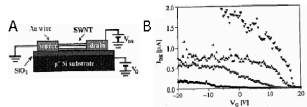
Fig. 17. A self-assembled SWNT-FET: A - schematic representation of the electrical measurement circuit; B - drain-source current versus gate voltage for different values of drain-source bias.
