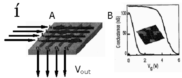
Fig. 16. A 4 by 4 crossed NW-FET array. A - with four horizontal NWs ( I_1 to I_4 ) as inputs and four vertical NWs ( O_1 to O_4 ) as signal outputs; B - conductance versus gate voltage of a single cNW-FET.
