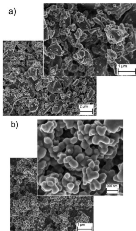
Fig. 1. Al_2O_3 ceramic powders: M, 660 nm (a) and TM, 135 nm (b)
